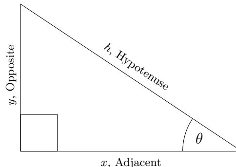
Figure 5.17: A right triangle
